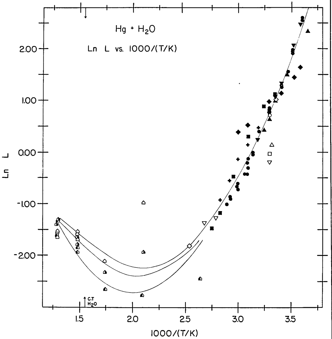
Figure 5. Mercury + Water, \ln L vs. 1000/(T/K) .
