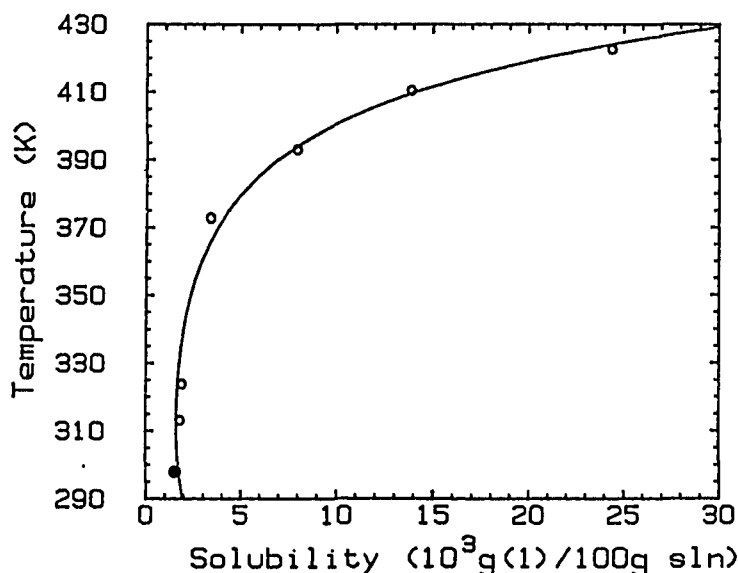
FIGURE 1. Solubility of methylcyclohexane in water : ref 4 (o); average of ref 3, 4 & 6 (●).
