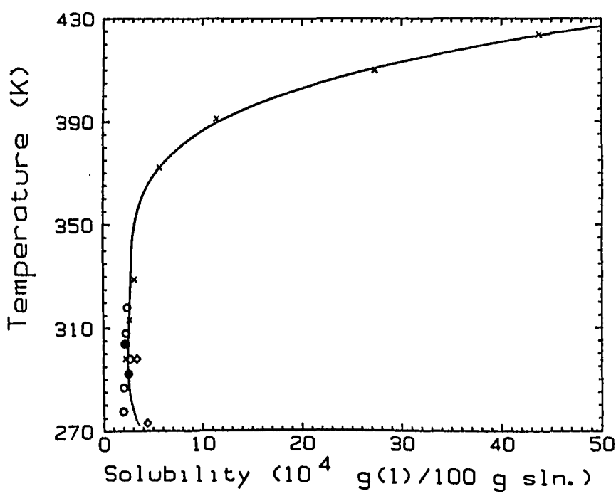
FIGURE 1. Solubility of heptane in water; selected data: ref 13 (o); ref 16 (◊); ref 18 (x), ref 23 (●).
