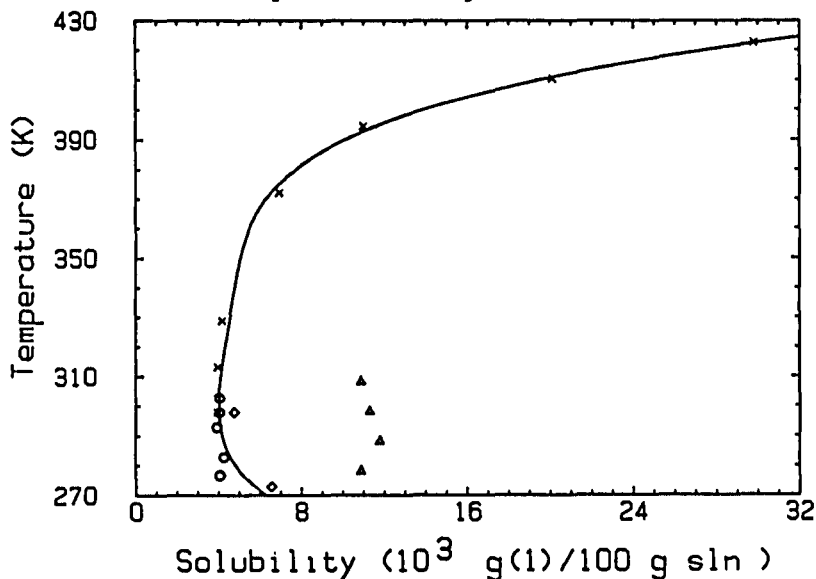
FIGURE 1. Solubility of pentane in water: ref 13 (x); ref 9 (o); ref 11 ( \diamond ); ref 10 ( \Delta , rejected data, see text). (continued)
