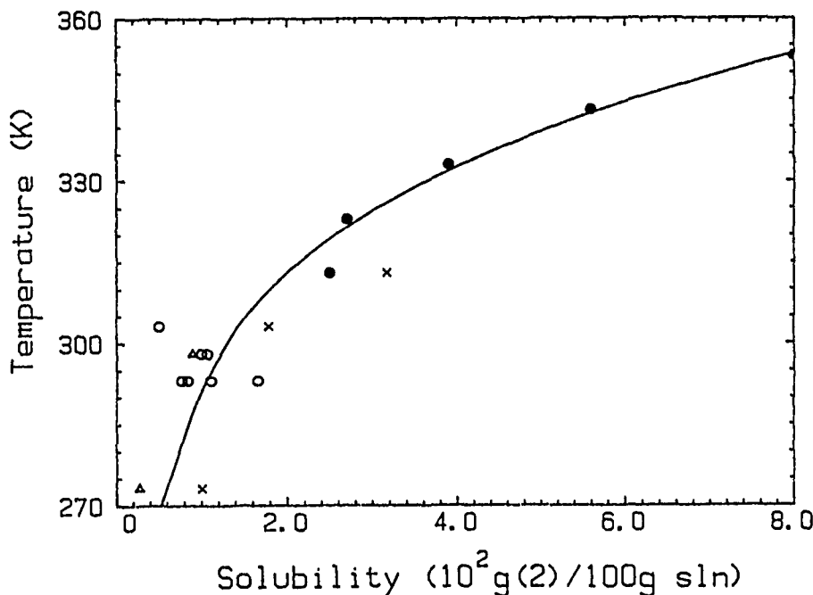
FIGURE 2. Solubility of water in hexane: ref 14 (x); ref 25 (Δ); ref 40 (●); other data (O). Line of best fit calculated for averaged "Best" values, see text.
