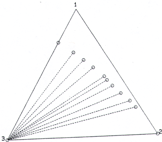
FIG. 46. Phase diagram of the system 1-octanol (1)—hexane (2)—water (3) at 293.2 K. ○—experimental data, Ref. 1, dashed lines—experimental tie lines, Ref. 1.
